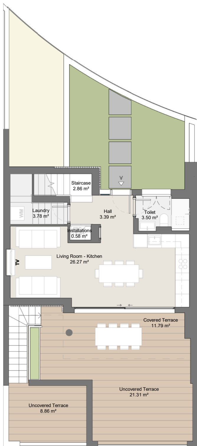
GROUND FLOOR
