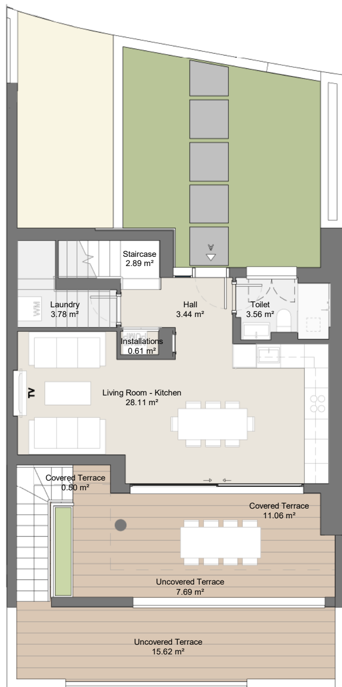
GROUND FLOOR
