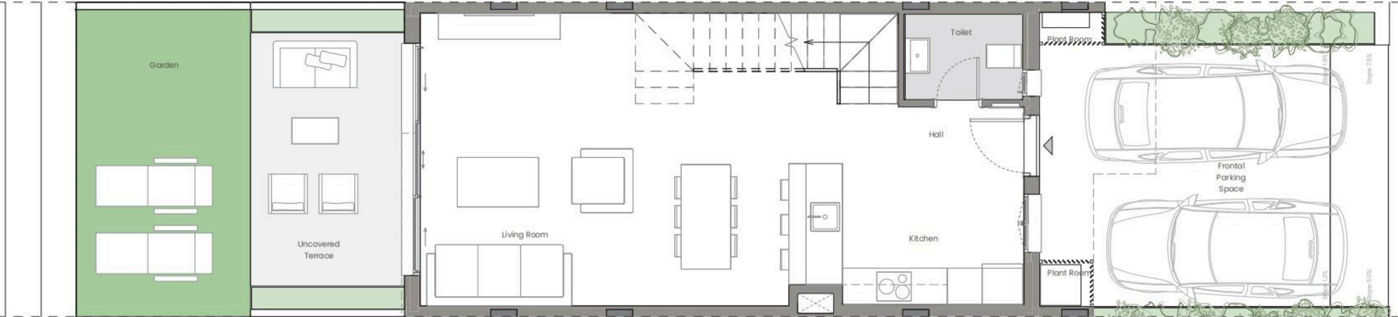
GROUND FLOOR
